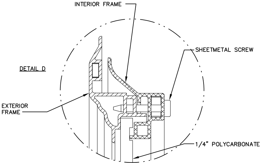
IMPACT WINDOW / ALUMINUM FRAME WITH GROOVED POLYCARBONATE DETAIL E
